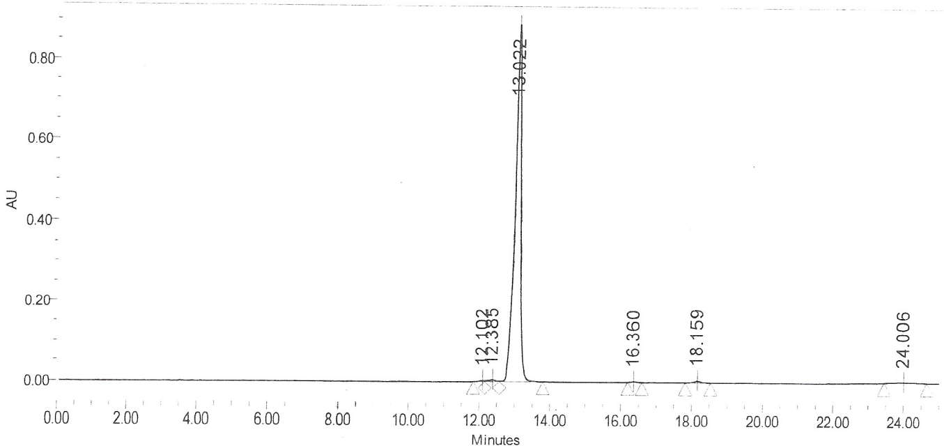
Auto-Scaled Chromatogram
